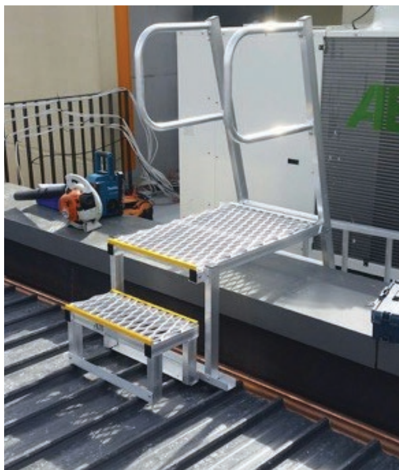
Single step installed for access from roof deck to ladder platform.
